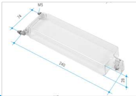
COIN ACCEPTOR SPLASH GUARD. TRANSPARENT PLEXIGLASS LARGE
