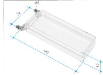
COIN ACCEPTOR SPLASH GUARD. TRANSPARENT PLEXIGLASS. SHORT
